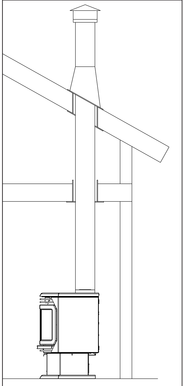
Figure 16: Straight vertical installation.
