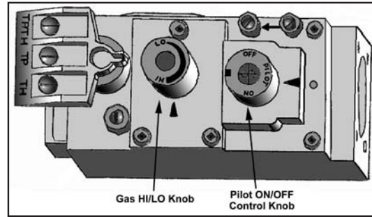
Figure 4: Gas Valve.
