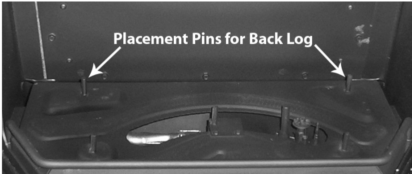
Figure 20: Step 1 of Log Placement.
