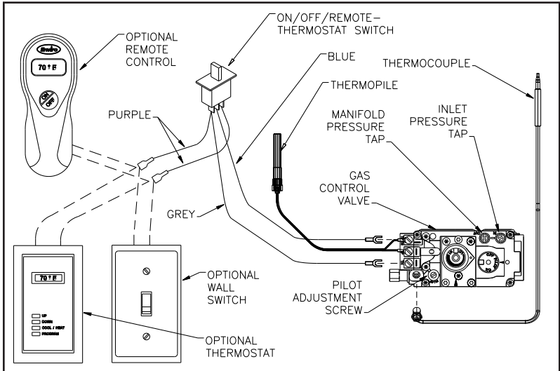
Figure 18: Wiring of a Thermostat
