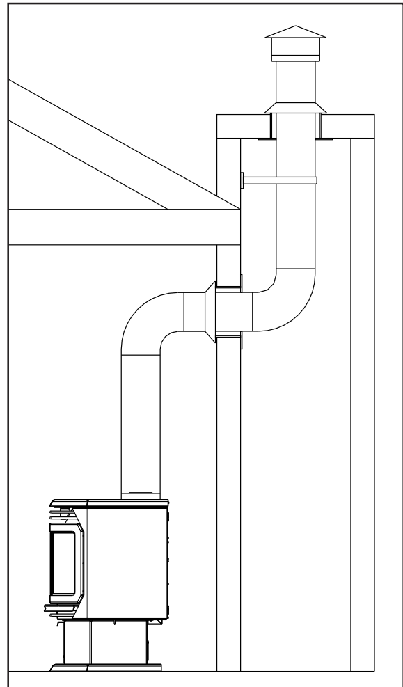
Figure 15: Installation into an existing chimney.
